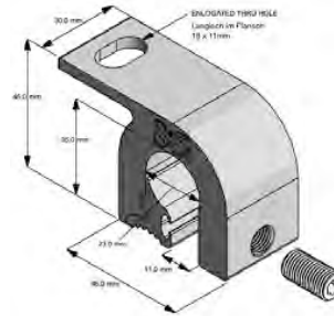
S-5!® Z-Mini-FL
